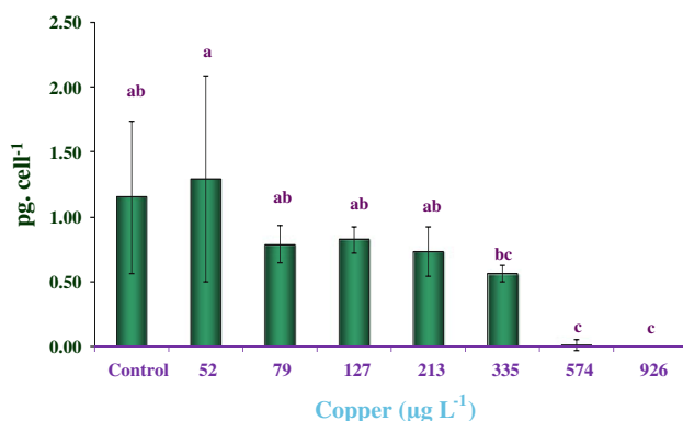
Fig. 2 Effect of Copper on chlorophyll a after 72 h exposure
