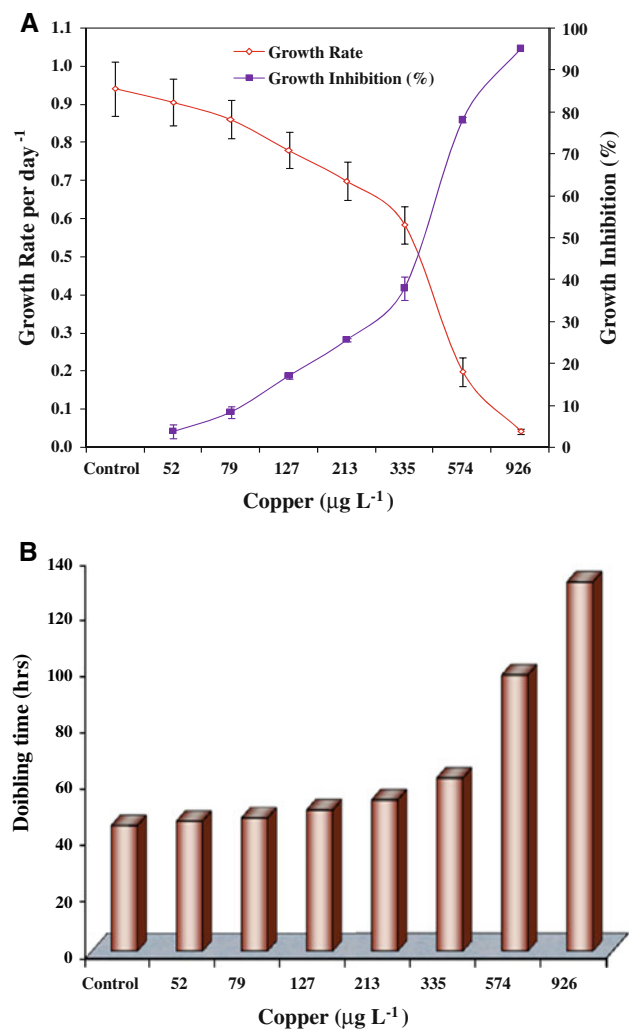
Fig. 1 a, b Dose-Response (growth rate, growth inhibition & doubling time) curve for the effect of copper (based on measured concentrations) on O. mobiliensis for 72 h exposure
