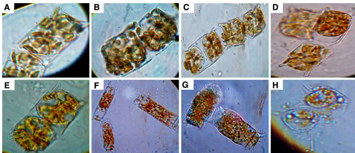
Fig. 4 Microscopic photographs of O. mobiliensis cells after exposure to different concentrations of copper for 72 h. a Control, b 52, c 79, d 127, e 213, f 335, g 574 and h 926 ( \mu\text{g Cu L}^{-1} )
