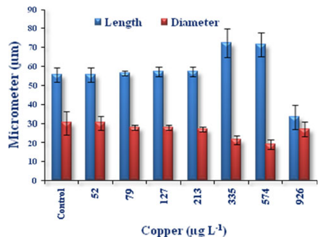
Fig. 3 Effect of Copper on cell size after 72 h exposure
